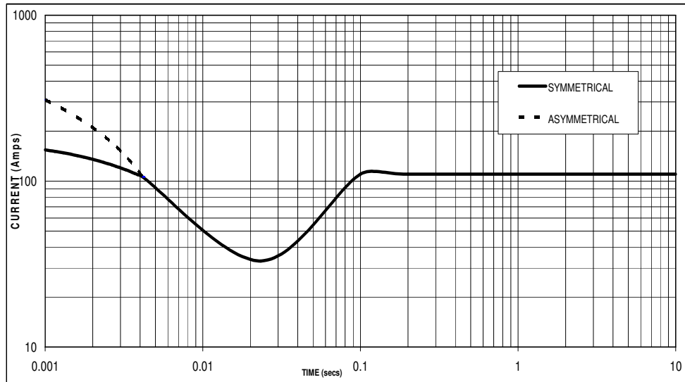
Sustained Short Circuit = 110 Amps
