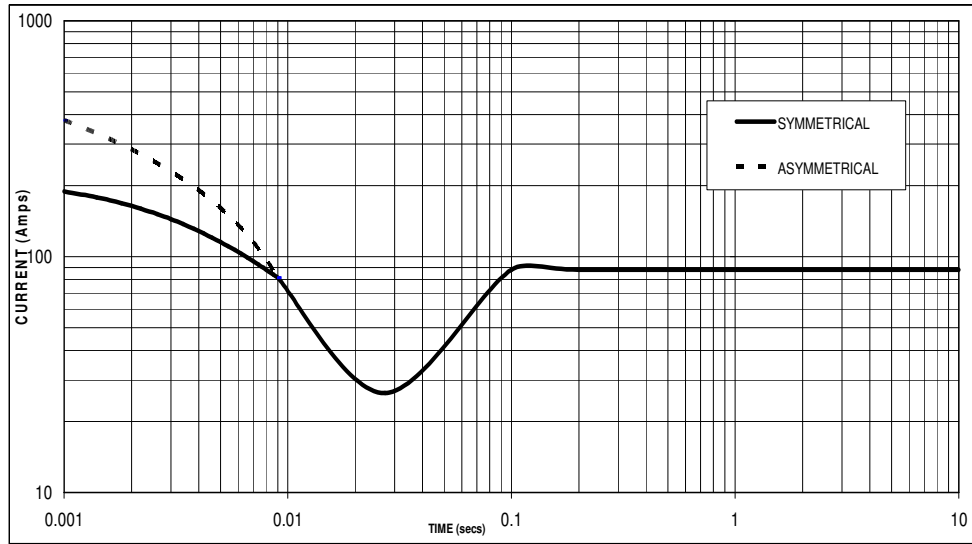
Sustained Short Circuit = 88 Amps
